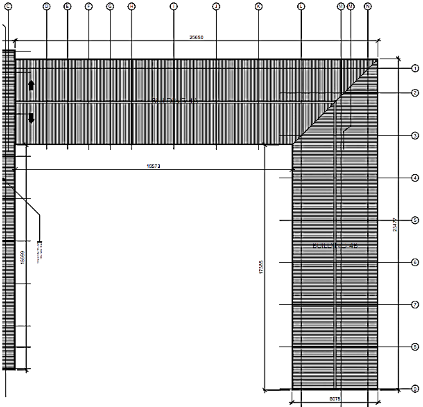
① Pnoc BLDG 4A & 4B ROOF PLAN
