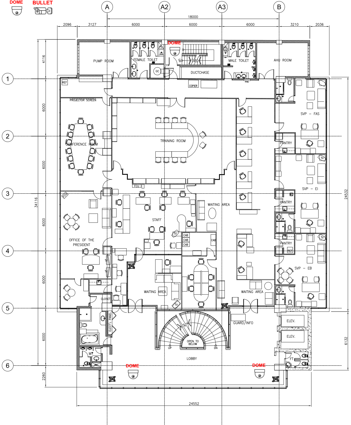
1 6TH FLOOR PLAN A-04 SCALE 1:100M
