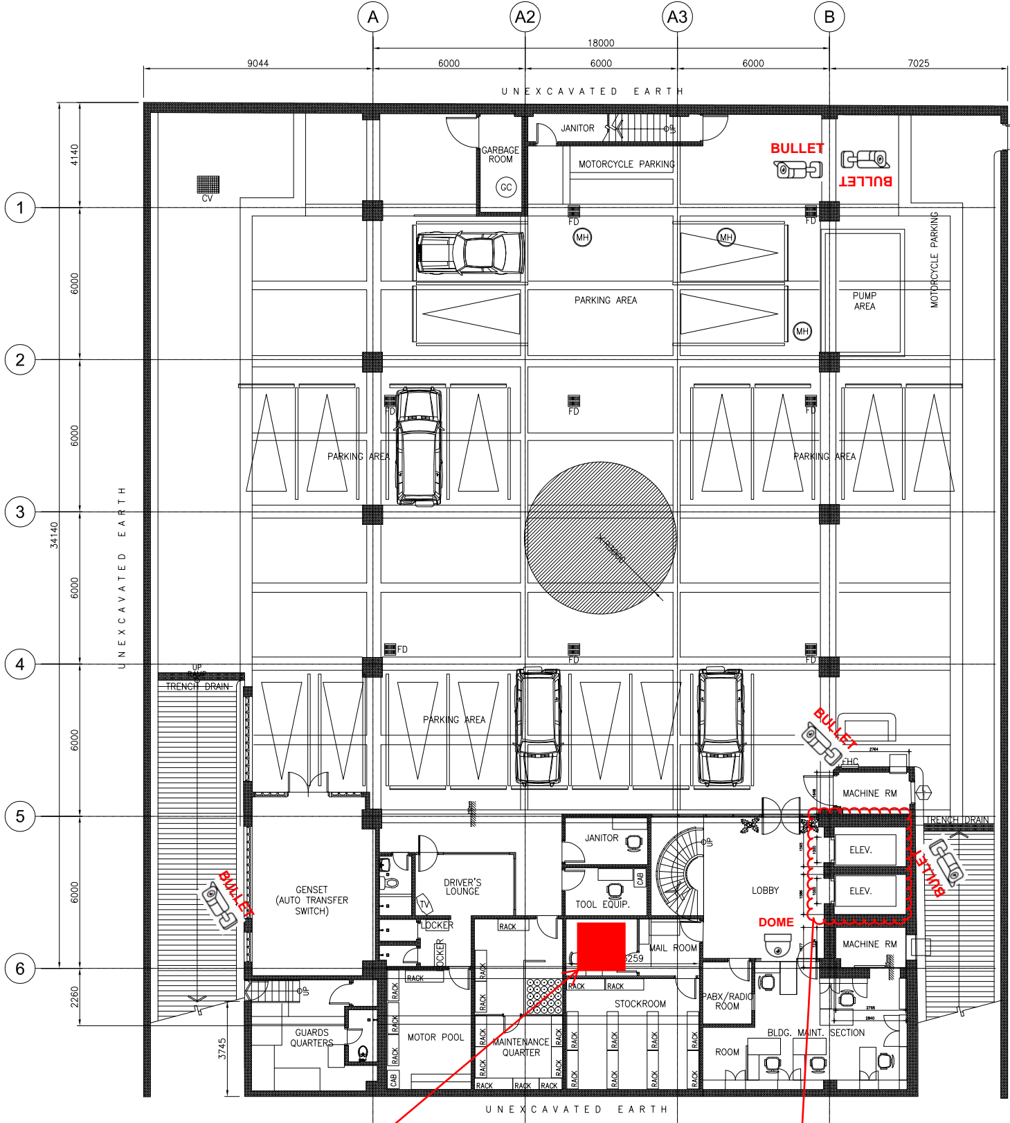
1 BASEMENT PLAN A-01 SCALE 1:100M
