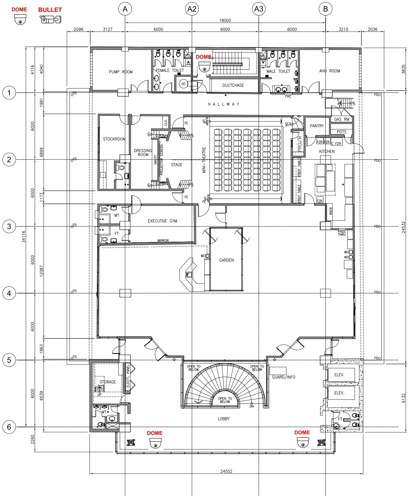
2 7TH FLOOR PLAN A-04 SCALE 1:100M
