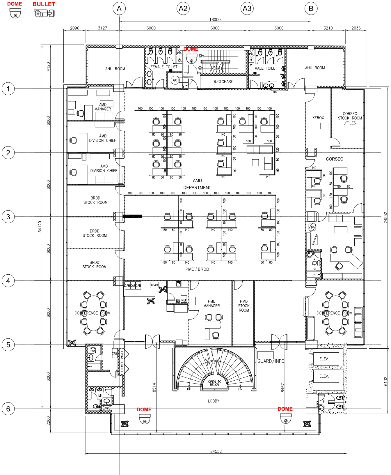
1 4TH FLOOR PLAN A-03 SCALE 1:100M
