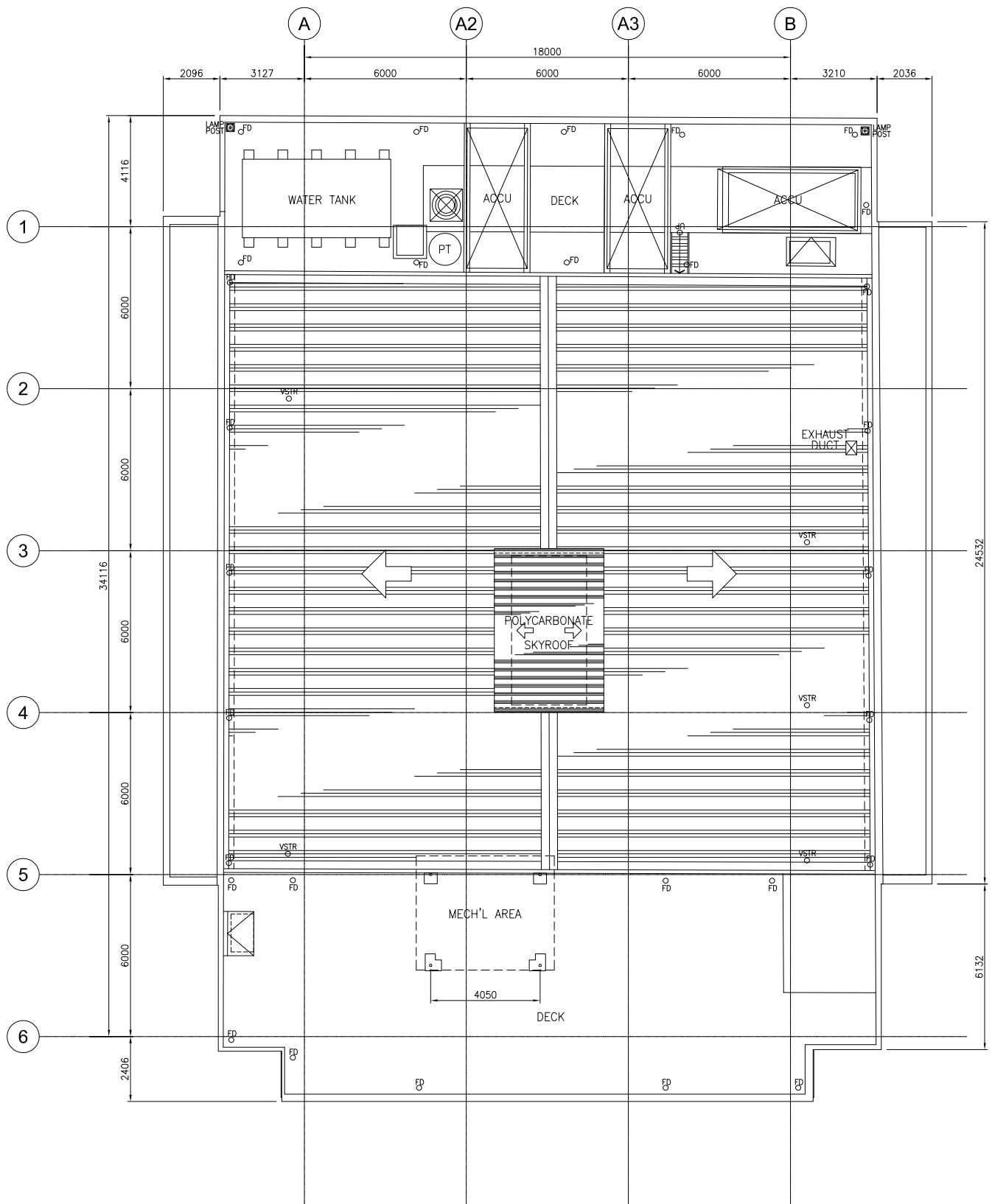
1 ROOF DECK PLAN A-05 SCALE 1:100M
