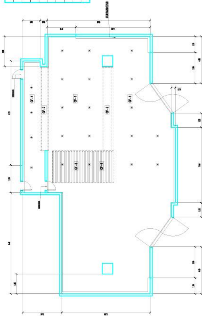
A 21 SCALE: 1:150m NETWORKING HALL 7TH FLOOR REFLECTED CEILING PLAN
