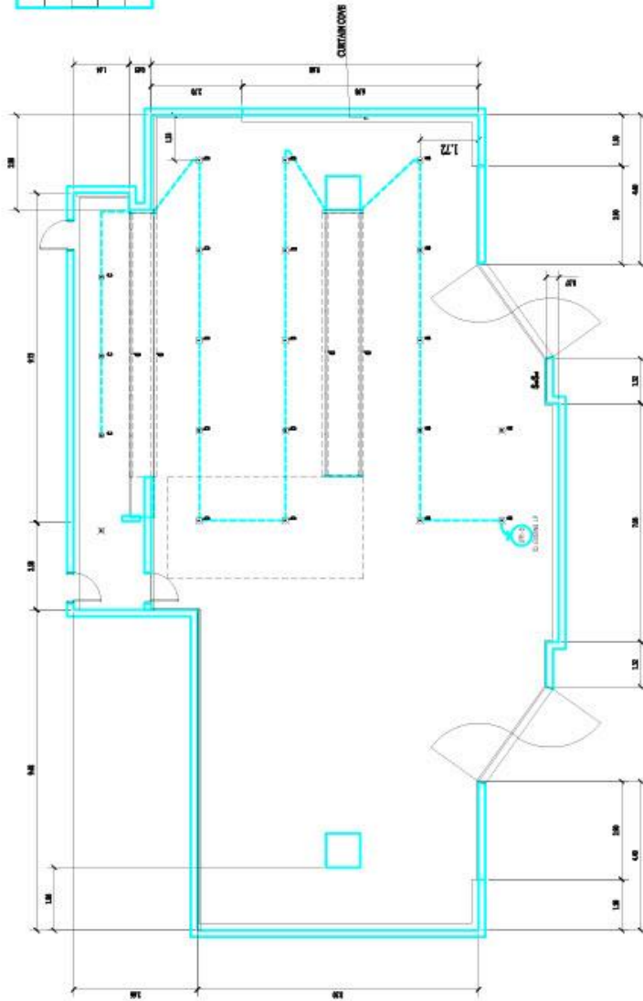
NETWORKING HALL 7TH FLOOR A LIGHTING LAYOUT SCALE 1:150m
