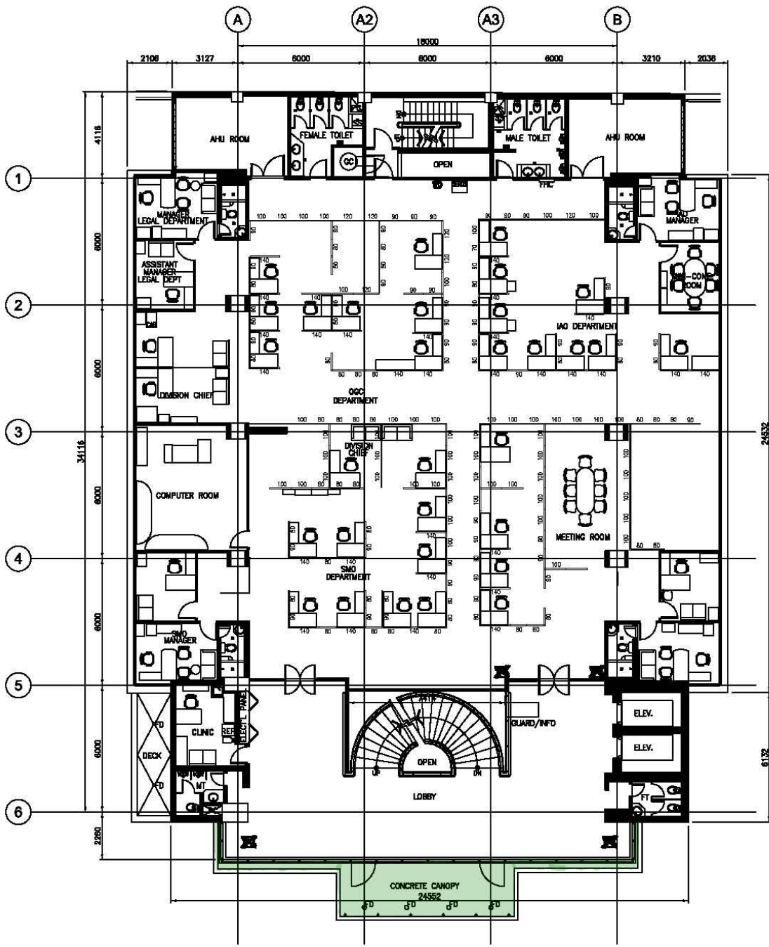
1 2ND FLOOR PLAN A-OZ SCALE 1:100M
