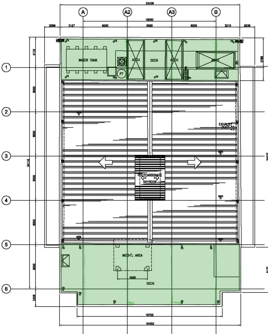
1 ROOF DECK PLAN A-05 SCALE 1:100M
