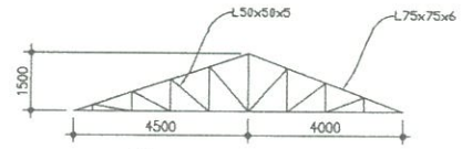
1 Truss 1, T1 A-01 SCALE
