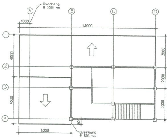
1 2ND FLOOR PLAN A-01 SCALE
