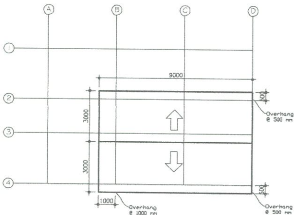
1 ROOF PLAN A-01 SCALE
