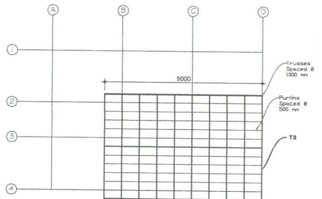
1 ROOF FRAMING PLAN 2 A-01 SCALE
