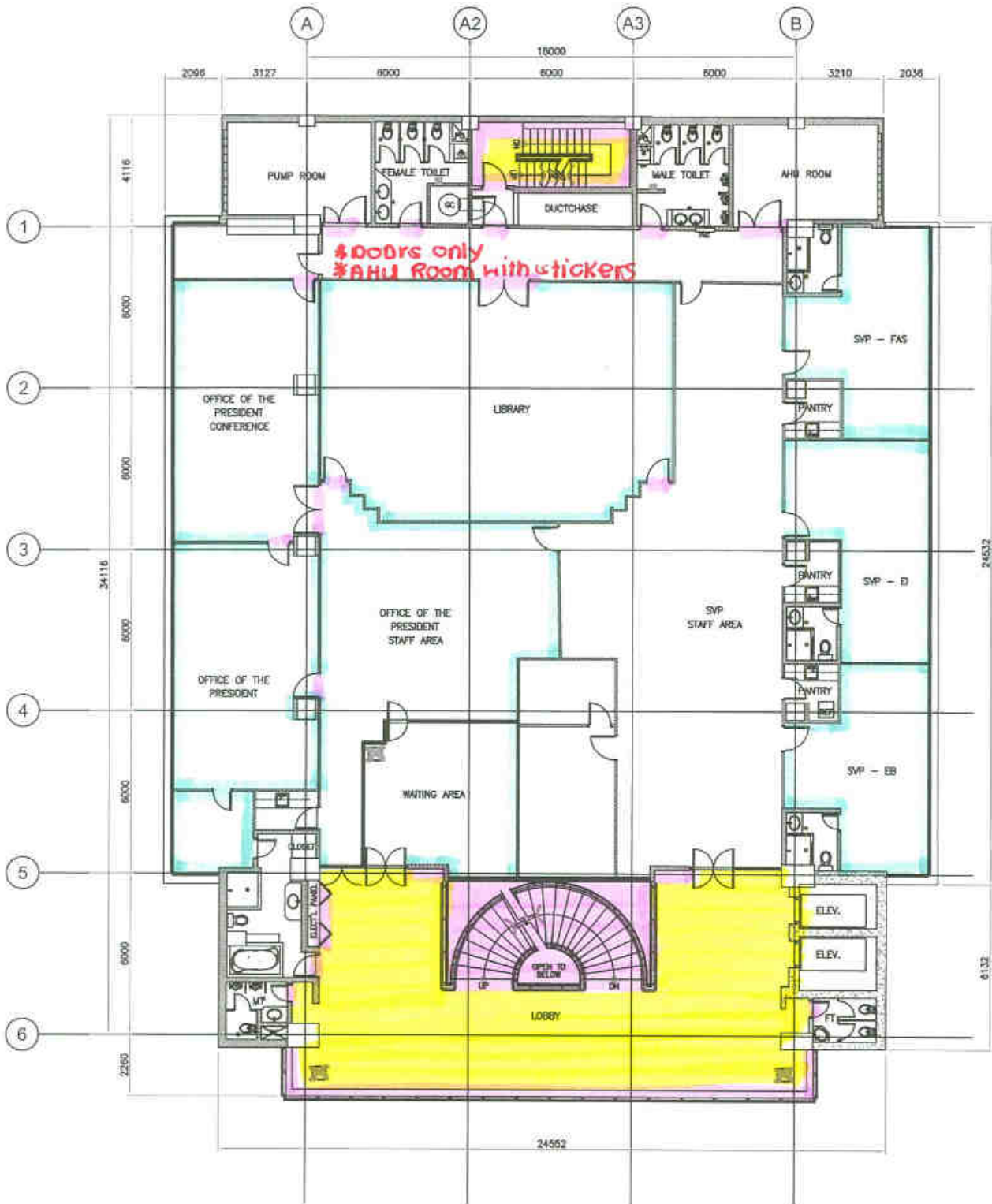
1 6TH FLOOR PLAN A-04 SCALE 1:100M
