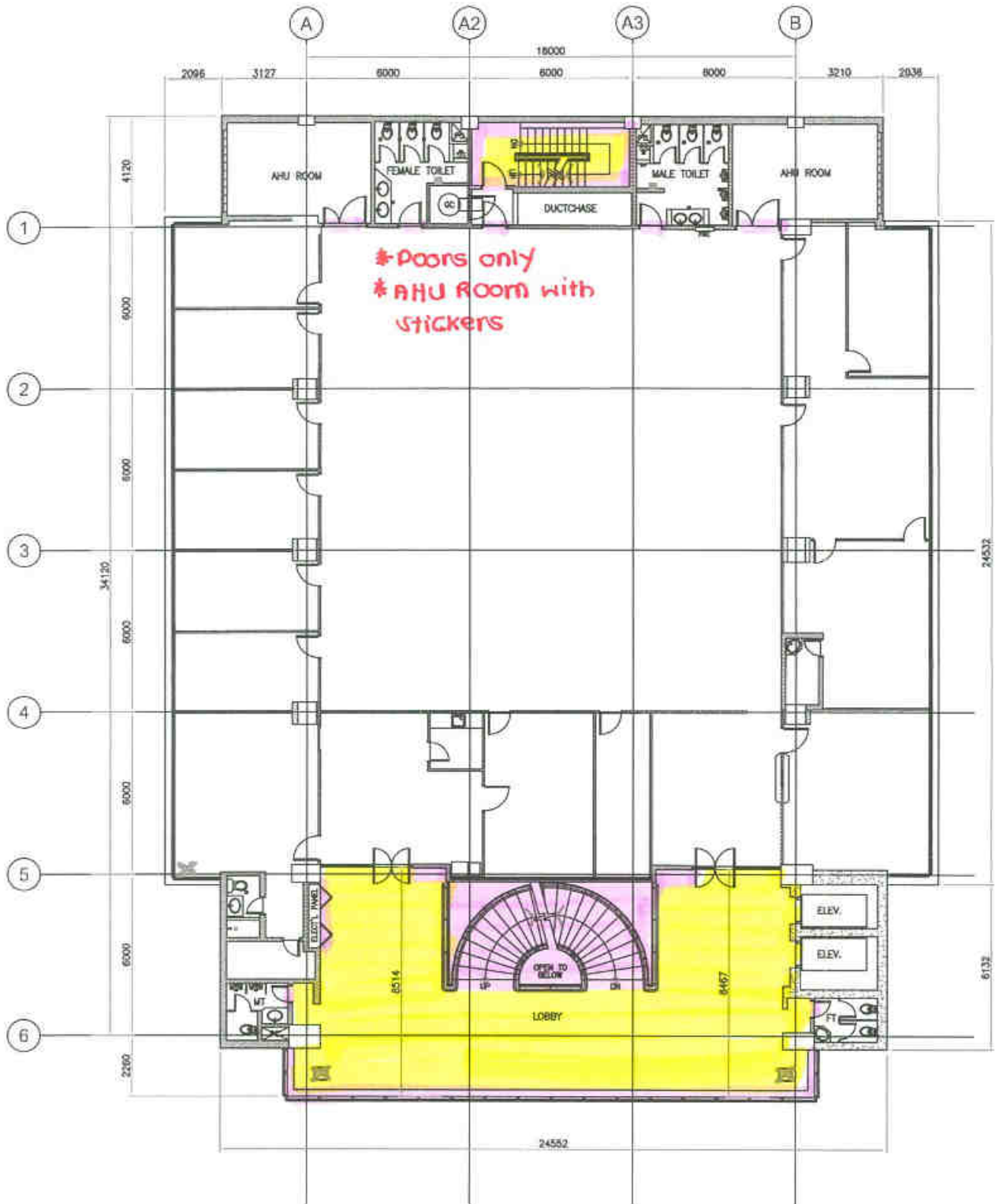
1 4TH FLOOR PLAN A-03 SCALE 1:100M
