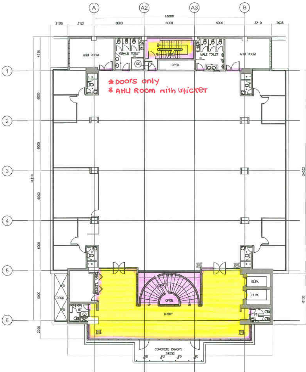
1 2ND FLOOR PLAN A-02 SCALE 1:100M
