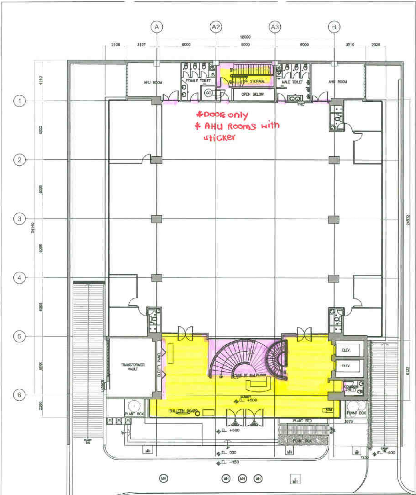
2 GROUND FLOOR PLAN A-01 SCALE 1:100M
