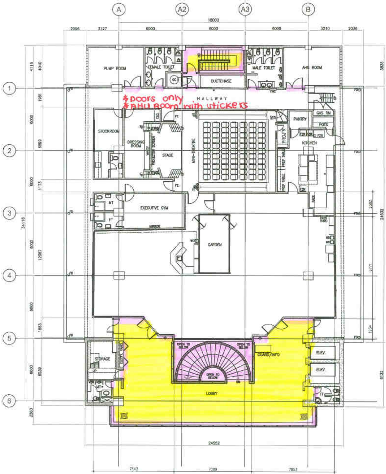
2 7TH FLOOR PLAN A-04 SCALE 1:100M
