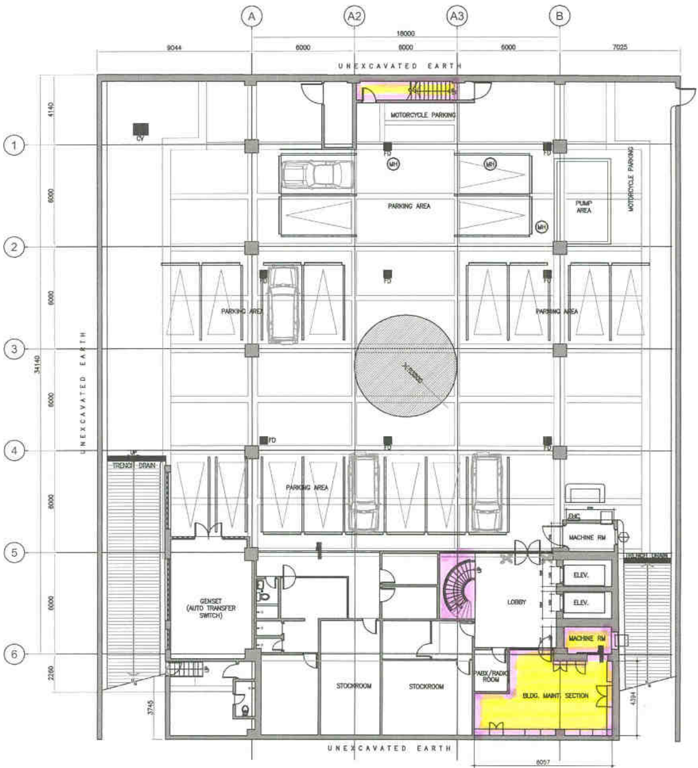
1 BASEMENT PLAN A-01 SCALE 1:100M
