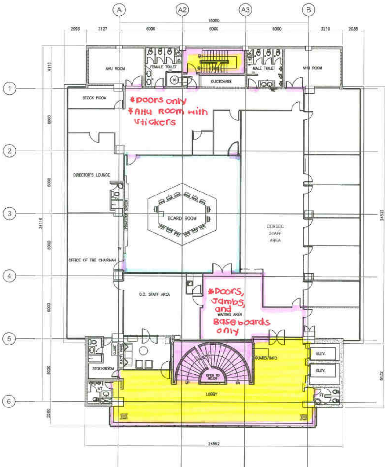
2 5TH FLOOR PLAN A-03 SCALE 1:100M
