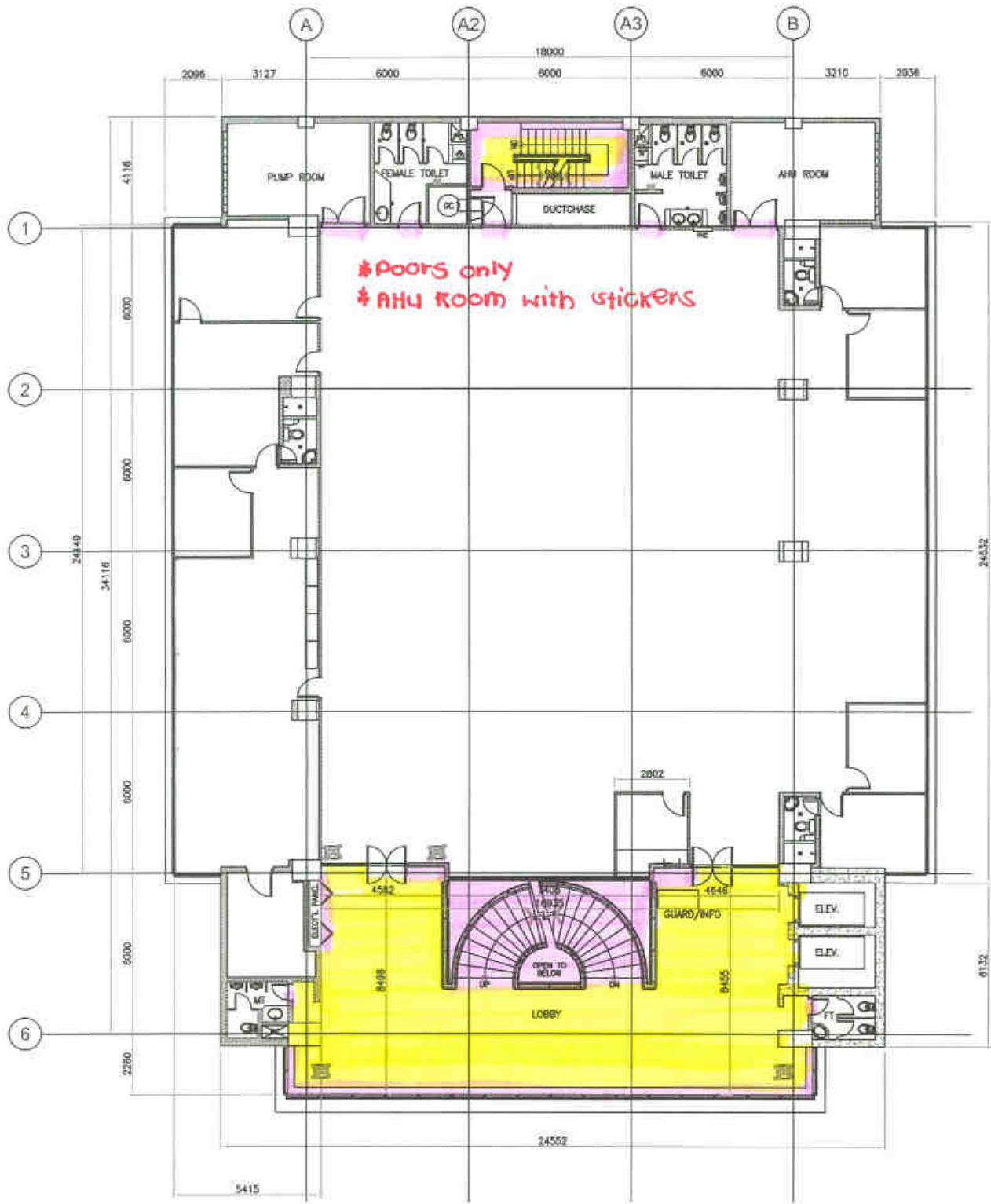
2 3RD FLOOR PLAN A-02 SCALE 1:100M
