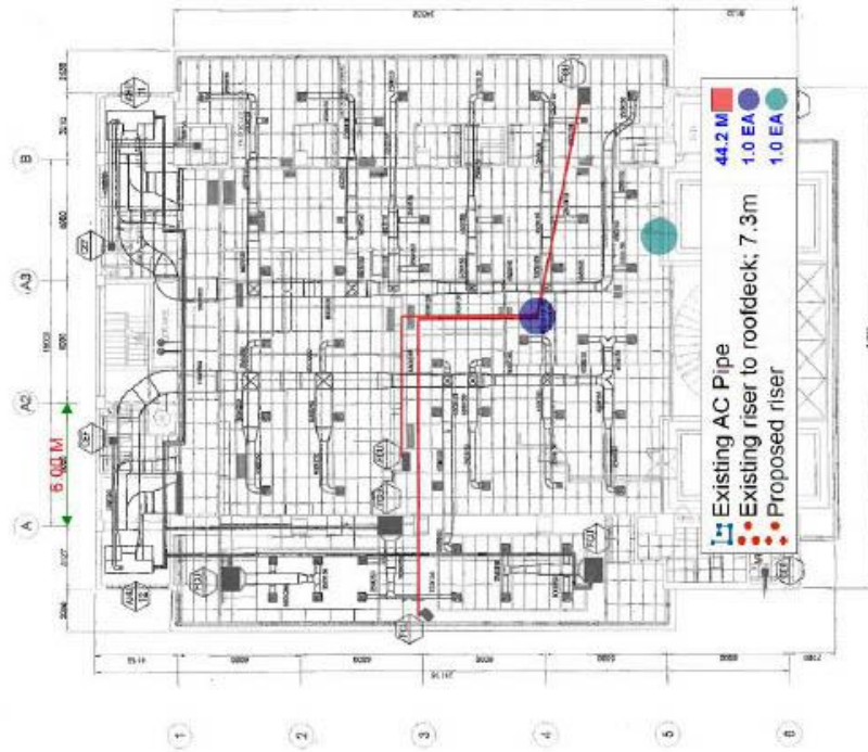
1. 6TH FLOOR A.C. & VENT LAYOUT 1:500
