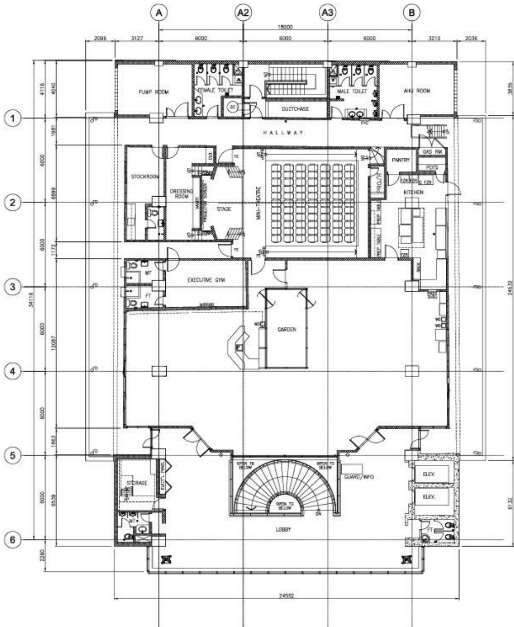
2 7TH FLOOR PLAN A-04 SCALE 1:100M
